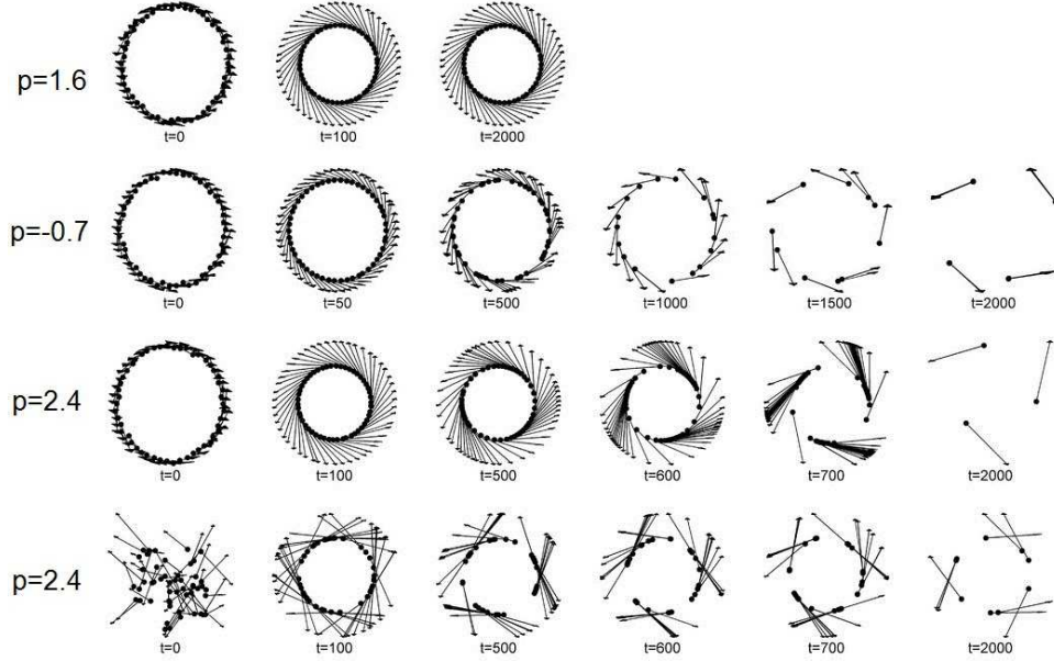
FIGURE 5. Dynamics of the 2nd order model (60) with N = 50 , g(s) = 1 - s^2 and f(r) = -r^p , with p as indicated. Row 1-3: The initial conditions are taken to be a slight random perturbation of a ring of radius one rotating counterclockwise. Row 4: Initial positions and velocities are taken to be random inside a unit square.
