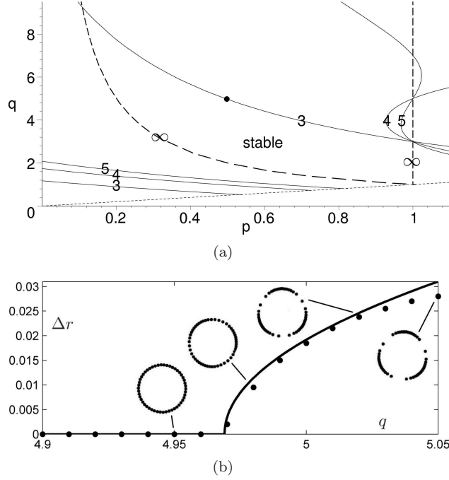
FIGURE 2. (a) Stability region of a ring solution for the force law (24). Instability boundaries corresponding to m = 3, 4, 5 and m = \infty are indicated. Crossing any of these boundaries triggers the corresponding instability. The stable region is bounded by the instability of mode 3 from above the curve pq = 1 (corresponding to instabilities of modes m \rightarrow \infty ) from below. (b) Bifurcation diagram for interaction force (24) near the dot shown in (a), with p = 0.5 , and as q is varied. The solid curve is derived from weakly nonlinear analysis while the dots are simulations of (2).
